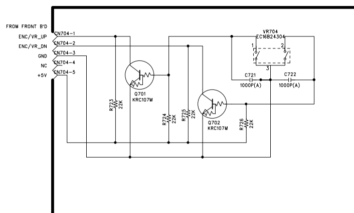
VOLUME SCHEMATIC
