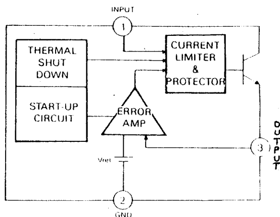
IC4, IC8, IC102, IC703 : KA78XX REGULATOR
