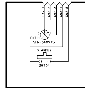
ST/BY SCHEMATIC
