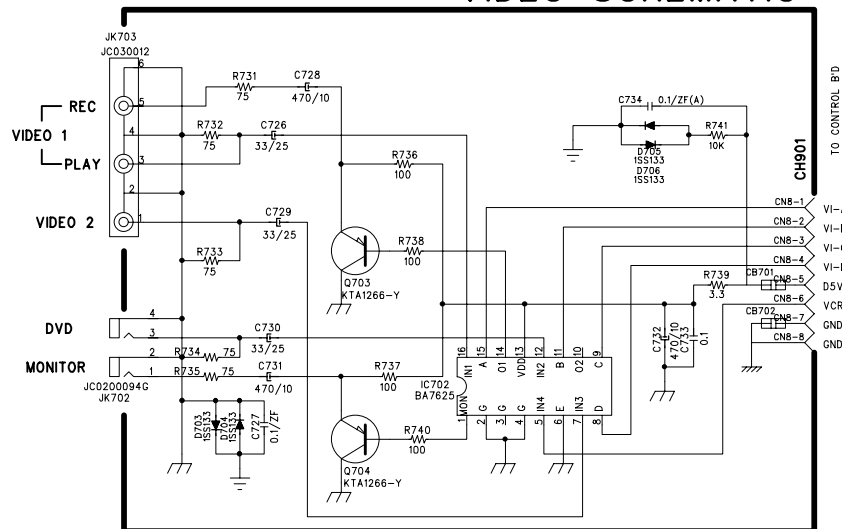
VIDEO SCHEMATIC
