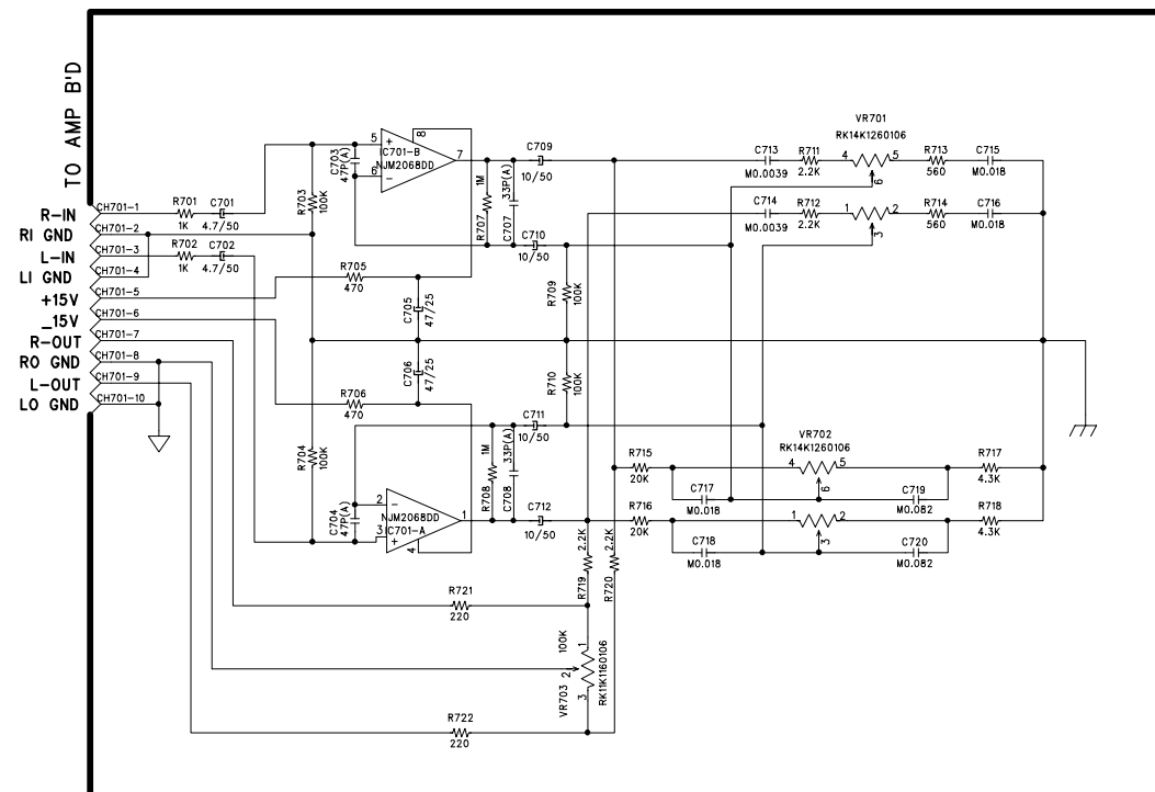
TONE SCHEMATIC
