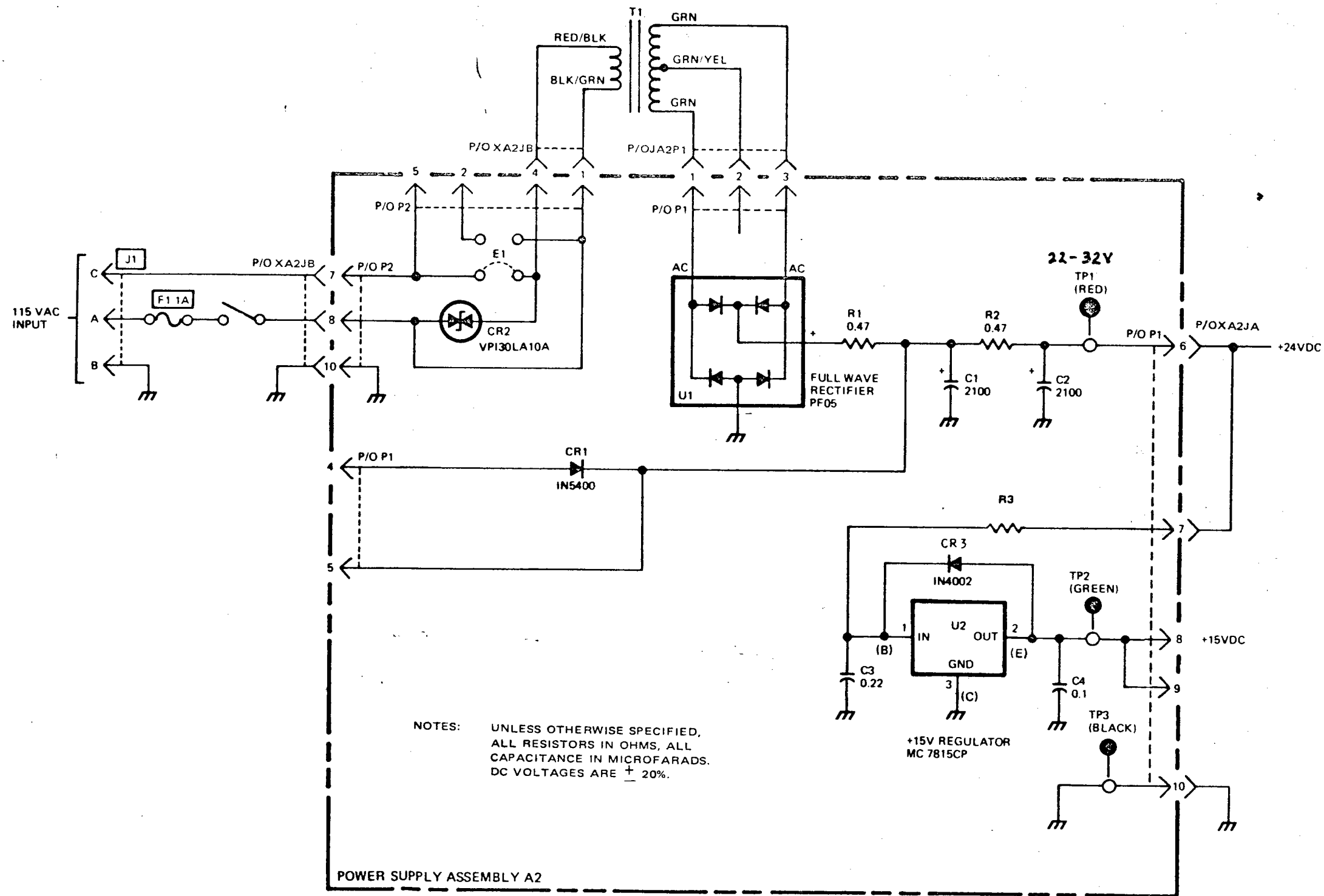
Figure 7-12. Power Supply IA2 Schematic Diagram
