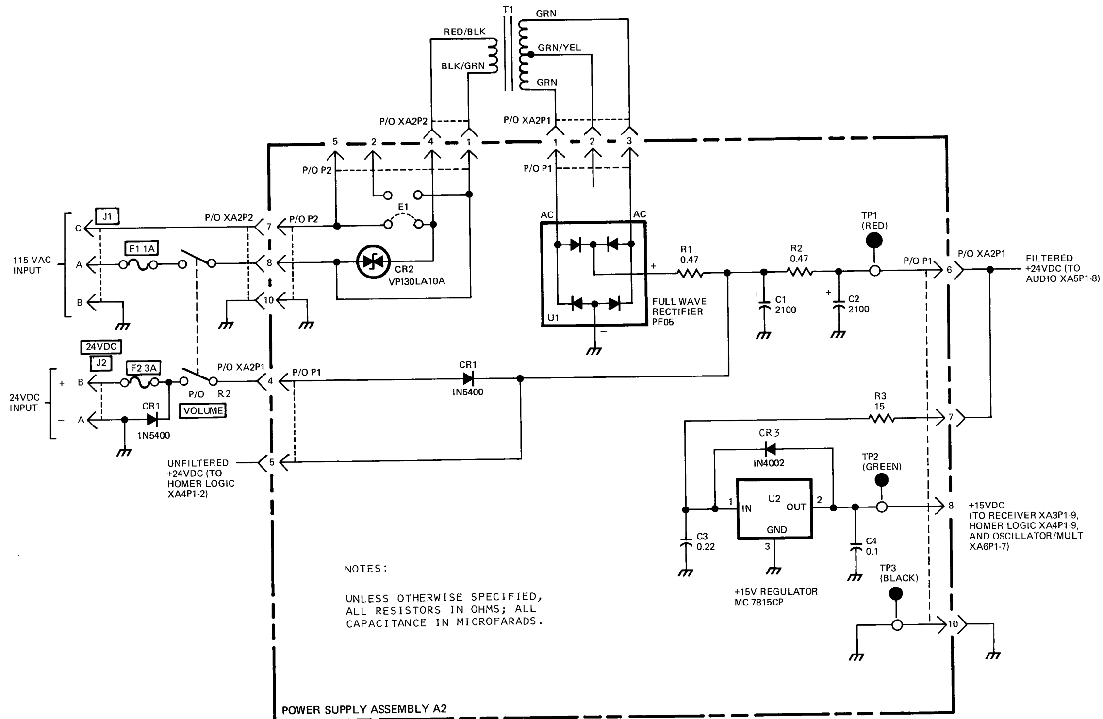
FIGURE 7-12. POWER SUPPLY 1A2 SCHEMATIC DIAGRAM
