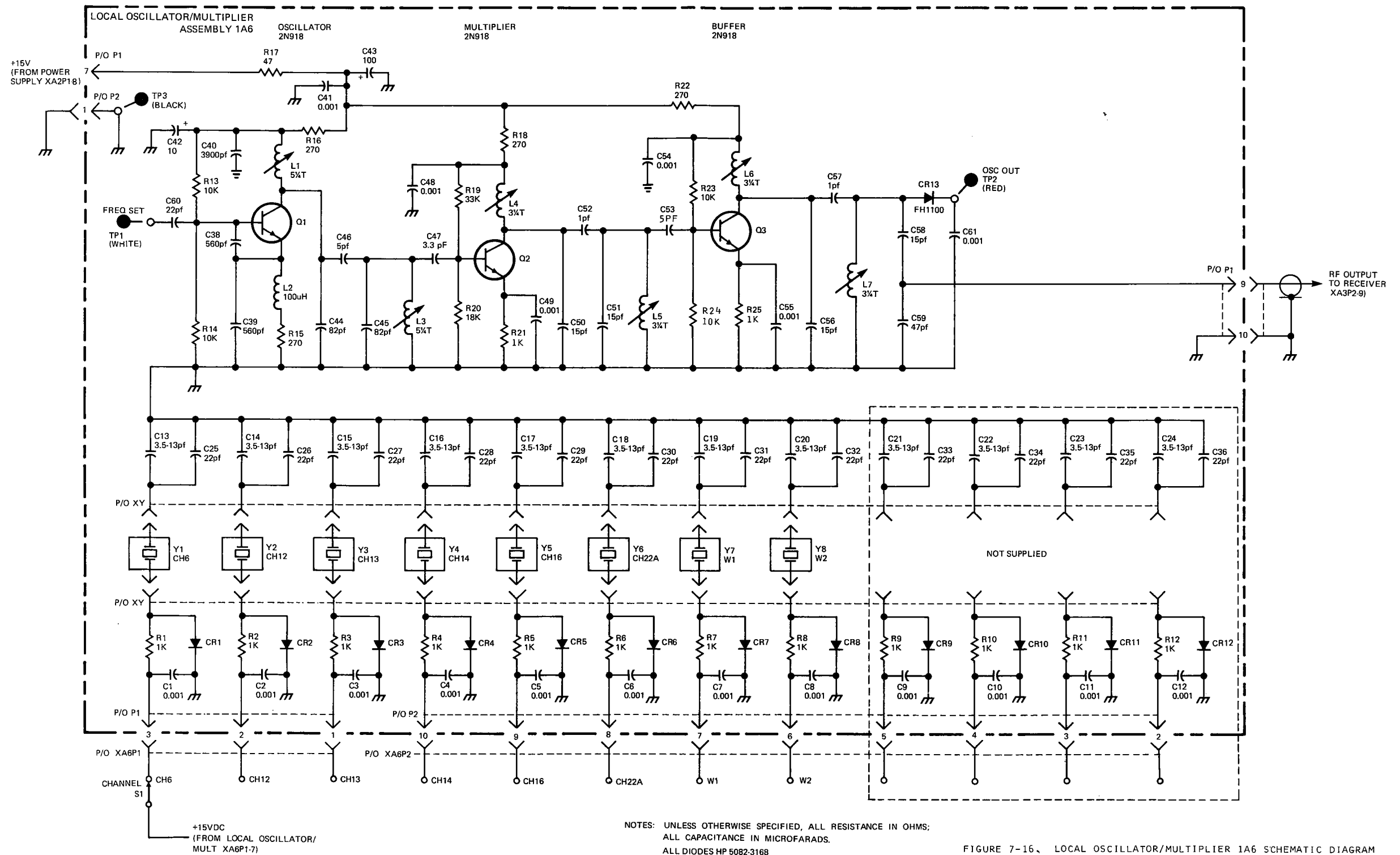
FIGURE 7-16. LOCAL OSCILLATOR/MULTIPLIER 1A6 SCHEMATIC DIAGRAM
