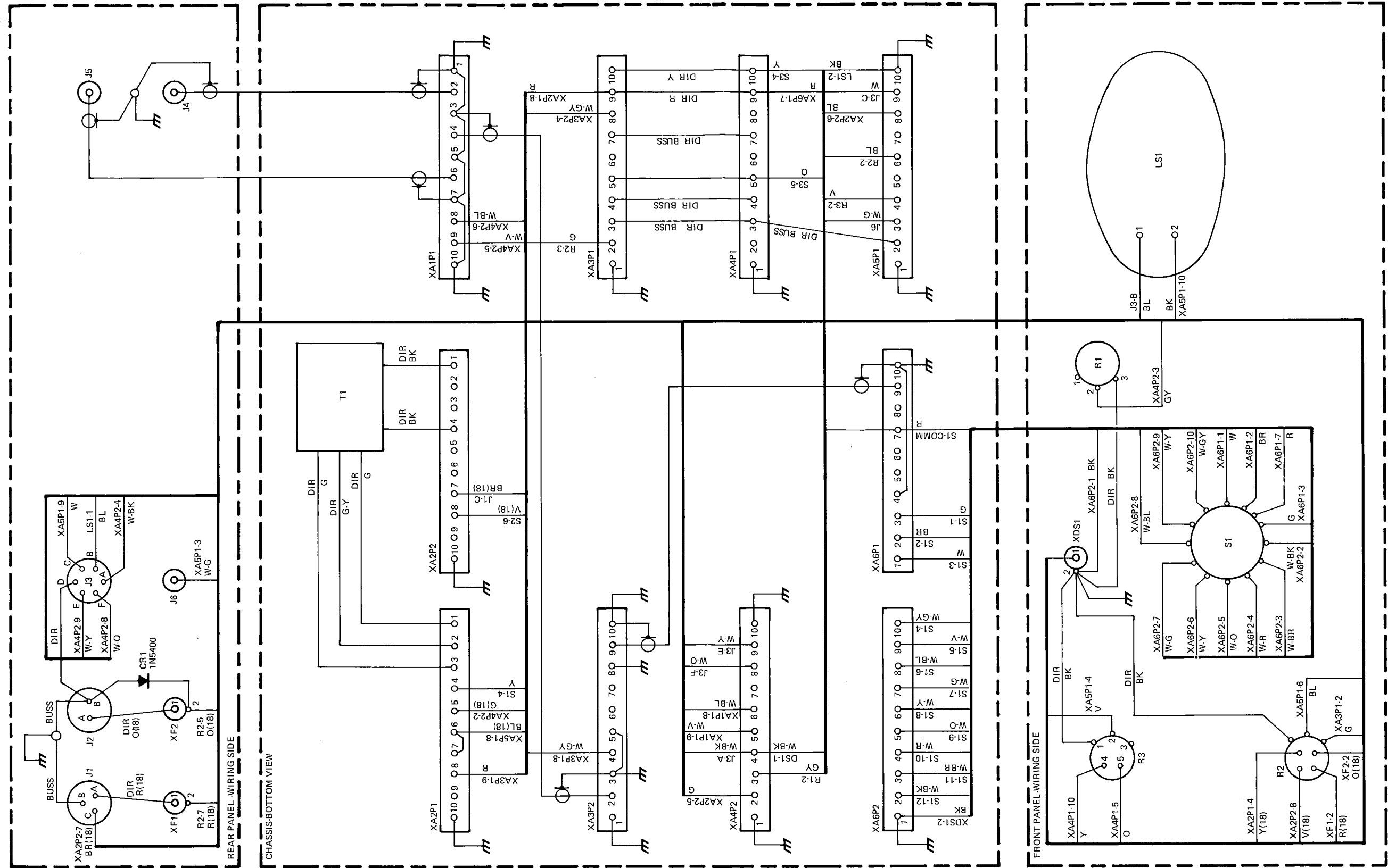
FIGURE 7-2. RECEIVER UNIT WIRING DIAGRAM
